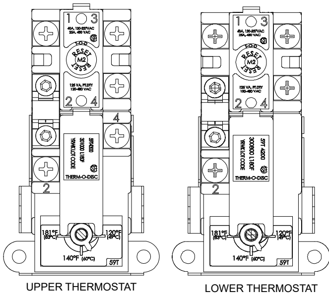
Figure 3. Thermostat Controls
