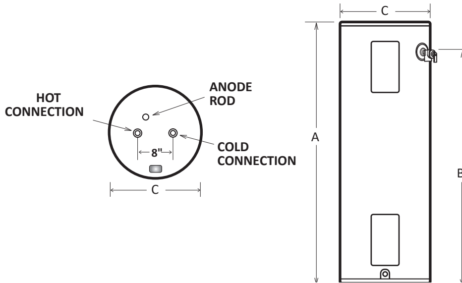
Figure 2. Rough-in Dimensions
