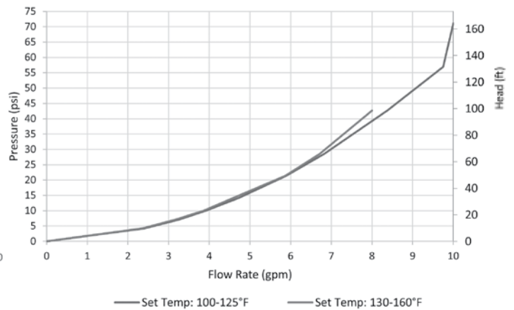
510CX3 PRESSURE LOSS
